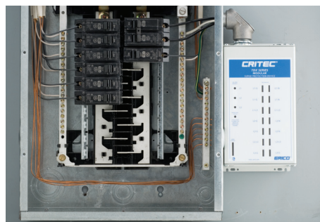
Typical installation
