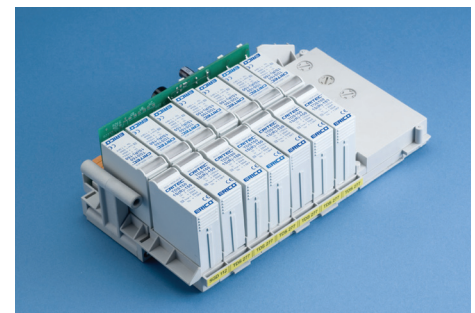
TDX Replaceable Module backplane fully removed
