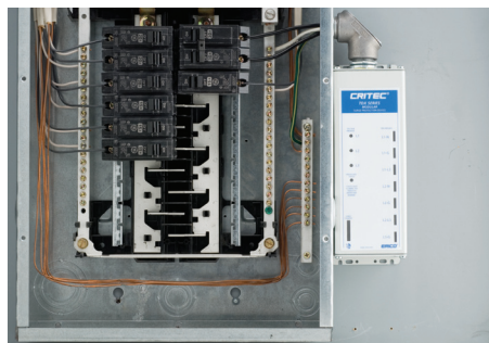
Typical Installation
